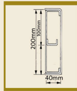
200x40mm 2 compartment (100/100)
