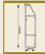
200x40mm 3 compartment (50/100/50)
