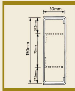
150x50mm 3 compartment (37.5/75/37.5)
