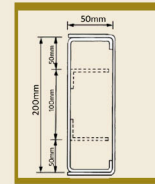
200x50mm 3 compartment (50/100/50)
