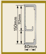
150x40mm 2 compartment (112/38)
