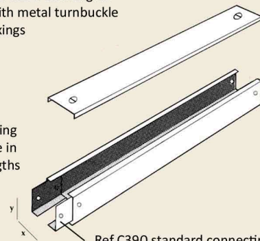
Ref C390 standard connecting sleeves. 1 pair supplied free of charge with each length of trunking. Now supplied with built in thread for increased speed of fixing
