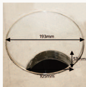
193mm diameter trimless
